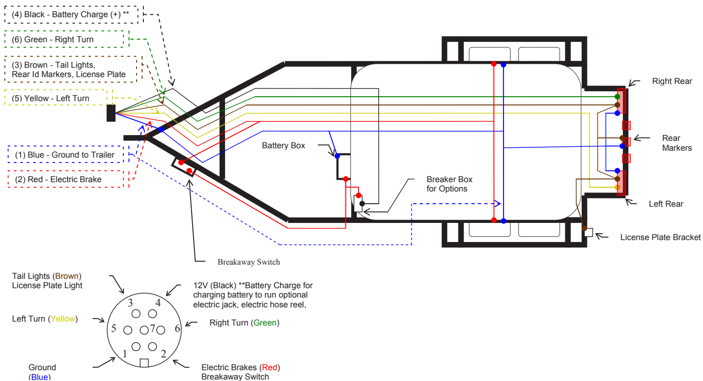
7-Pole Trailer Connector
